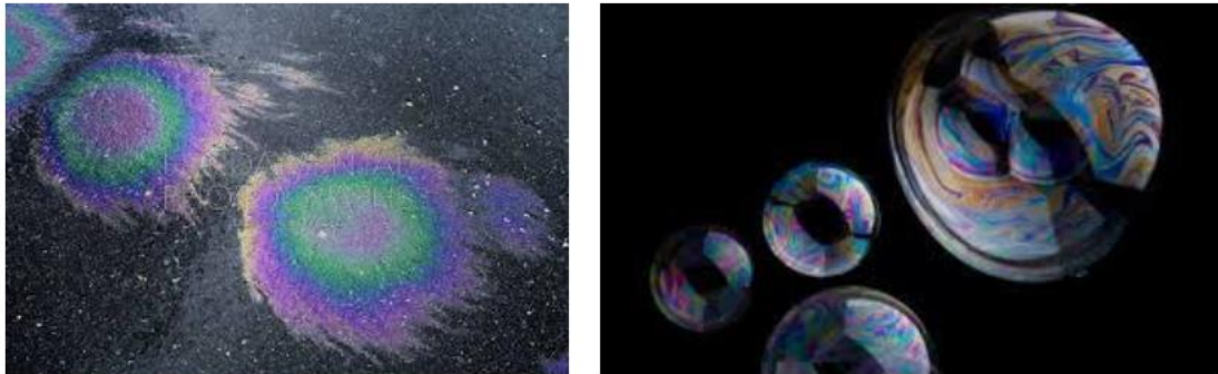
Figure 2. Oil spots on water ( www.fphoto.com , left) and soap bubbles ( www.sparticle.org , right).
