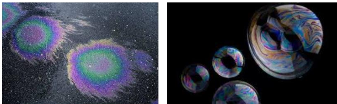
Figure 2. Oil spots on water ( www.fphoto.com , left) and soap bubbles ( www.sparticle.org , right).
