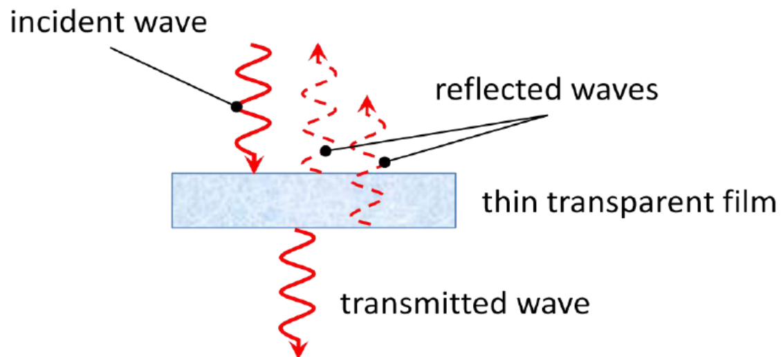
Figure 1. Interference in a thin film.
