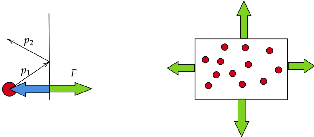
FIGURE 1. Left figure: if a molecule (red ball) collides with a container wall, molecule's momentum is changed from p_1 to p_2 . Therefore wall acted on it with some force (shown in blue) and by Newton's third law the molecules acts on the wall with an equal force F (shown in green). Right figure: Force of pressure acting on a container wall is directed outwards on each wall. Note that magnitude of the force is larger for walls with bigger area: if pressure is the same, force grows with area.
