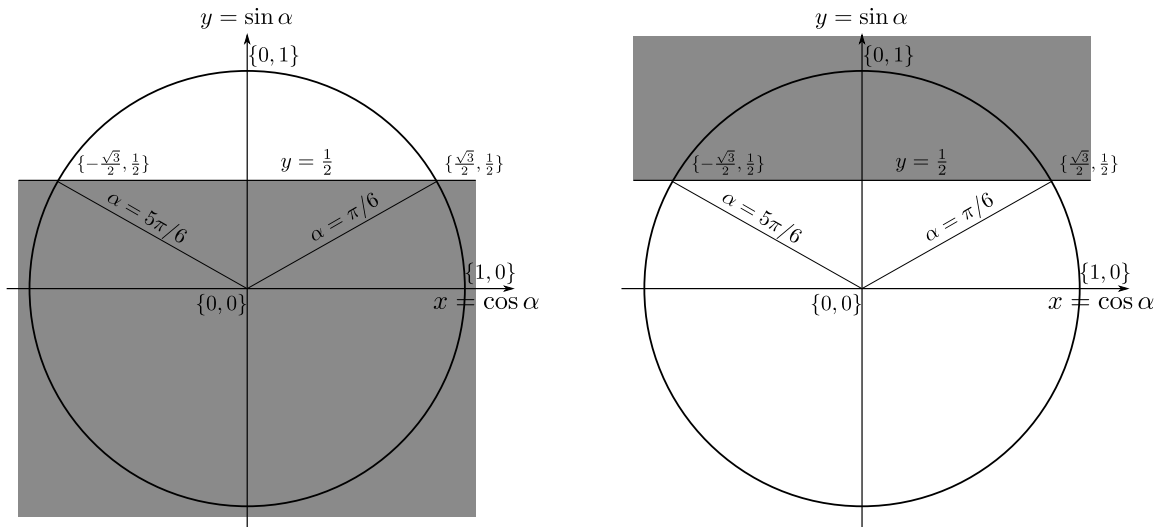
FIGURE 1. Solving equations \sin \alpha > \frac{1}{2} (left) and \sin \alpha < \frac{1}{2} (right): points on the circle in the unshaded regions satisfy the inequalities.
